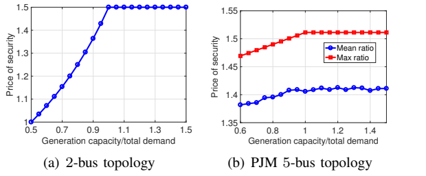
Fig. 3. PoS with fixed demand and different generation capacities
