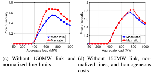
Fig. 7. Results of PJM 5-bus network with different values of demand
