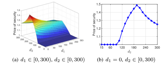
Fig. 4. PoS for 2-bus network in entire state space of demand distribution
